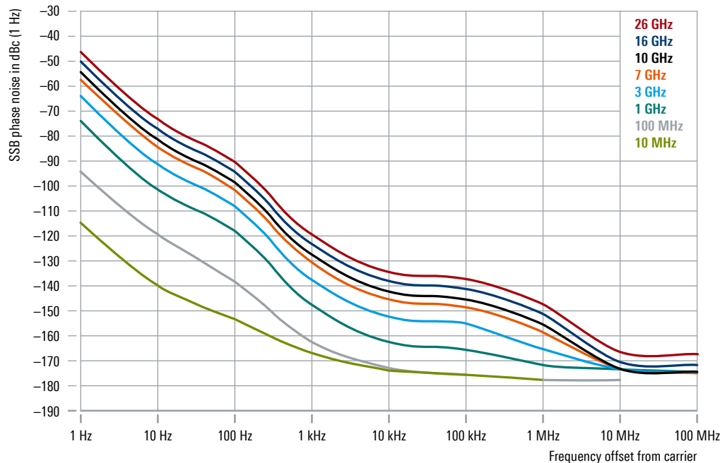
Typical phase noise sensitivity (correlation factor = 1, signal level = 10 dBm)
